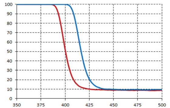
% HEV Filtered Standard Polycarbonate (red) vs Clear Blue Filter (blue)
